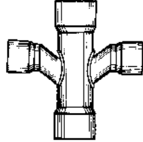
DOUBLE COMB. WYES & 1/8 BENDS SW x SW x SW
