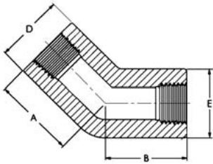
45° Elbow FPT x FPT
