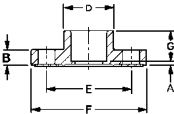
Flange Companion Soc
