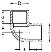
90° Elbow Soc x Soc
