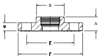
Flange Companion FPT
