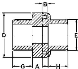
Union Soc x Soc with O-ring made of Viton®
