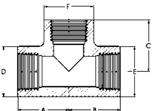
Tee All FPT
