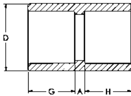
Coupling Soc x Soc
