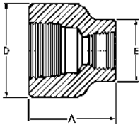
Female Adapter Soc x FPT
