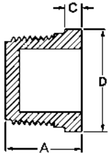
Flange Companion Soc
