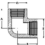
90° Elbow FPT x FPT
