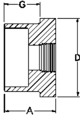
Reducing Bushing Spigot x Reducing FPT
