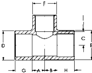
Tee Soc x Soc x FPT
