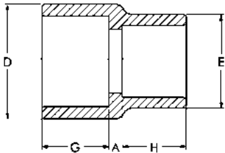
Coupling-Reducing Soc x Reducing Soc
