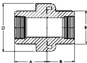
Union FPT x FPT with O-ring made of Viton®
