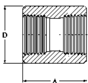
Coupling FPT X FPT
