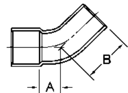
45° Street Elbow Fitting to Copper
