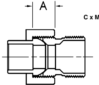
CxM Union Copper to Male NPT
