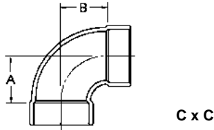
90° DWV Elbow Copper to Copper
