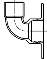
90° Flanged Sink Elbow Copper to Flange
