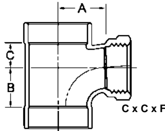
DWV-Female TY Copper to Copper to Female NPT
