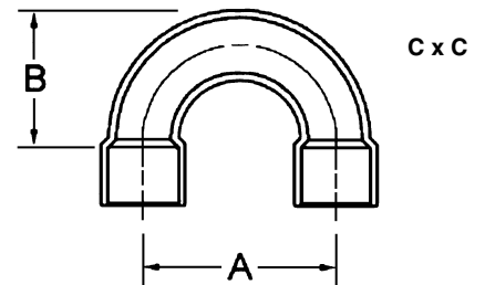
Return Bend Copper to Copper
