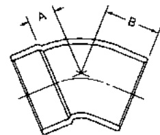
45° DWV Street Elbow Fitting to Copper
