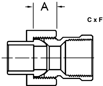
CxF Union Copper to Female NPT
