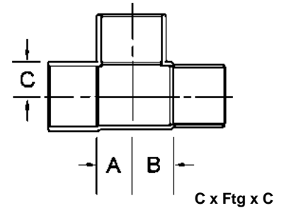
Street Tee Copper to Fitting to Copper
