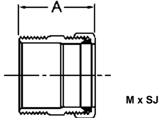
DWV-M x SJ Adapter Male NPT to Slip Joint
