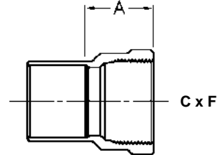
Female Adapter Copper to Female NPT
