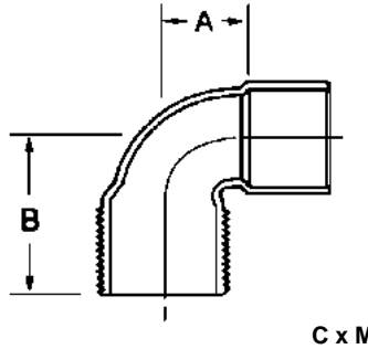
90° CxM Elbow Copper to Male NPT
