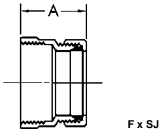
DWV-F x SJ Adapter Female NPT to Slip Joint
