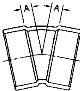
22-1/2° DWV Elbow Copper to Copper
