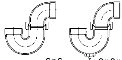
DWV- P Trap-Ground Swivel Joint Copper to Copper
