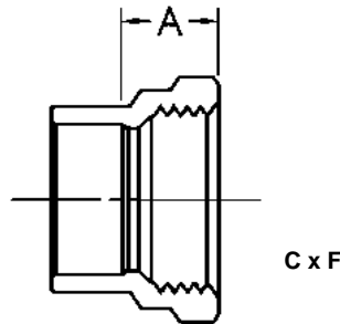
DWV-Female Adapter Copper to Female NPT
