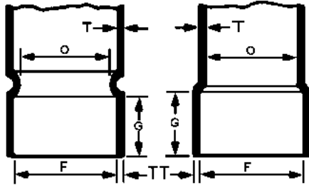
Female (Copper)
