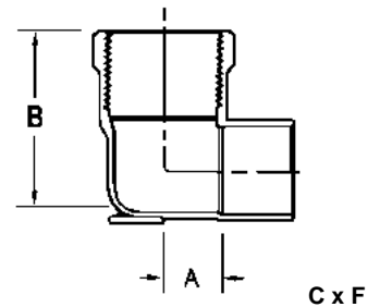
90° CxF Drop Ear Elbow Copper to Female NPT
