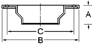
DWV-Closet Flange Copper to Closet
