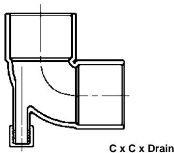
90° CxC Vent Elbow Copper to Copper to Drain Cap
