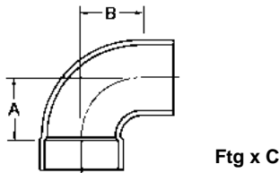
90° DWV Street Elbow Fitting to Copper
