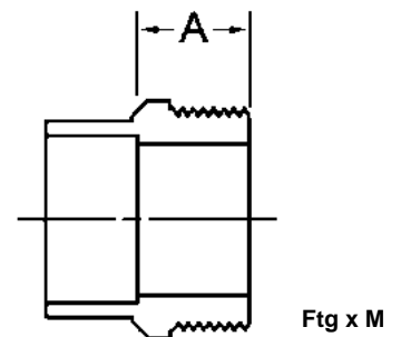
DWV - Ftg x M Adapter Fitting to Male NPT
