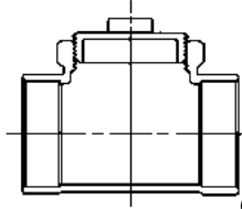
DWV-Line Cleanout (Test Tee) Copper to Copper Cleanout with Plug
