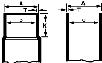
Male (Fitting)
