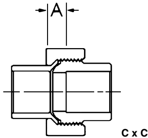
Union Copper to Copper
