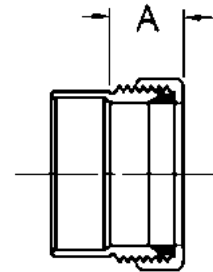
DWV-C x SJ Adapter Copper to Slip Joint
