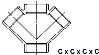
45° DWV Double Y Copper to Copper to Copper to Copper
