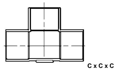
CxCxC Drop Ear Tee Copper to Copper to Copper
