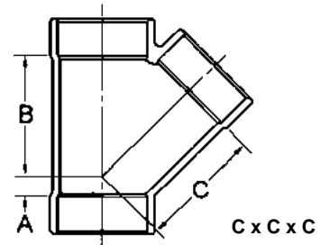
45° DWV Y Copper to Copper to Copper
