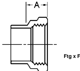
DWV-Ftg x F Adapter Fitting to Female NPT
