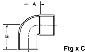
90° Street Elbow-Close Ruff Fitting to Copper
