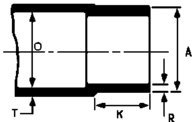
Male (Fitting)
