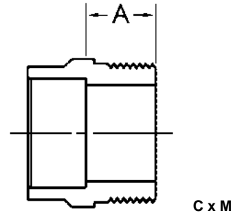
DWV-Male Adapter Copper to Male NPT
