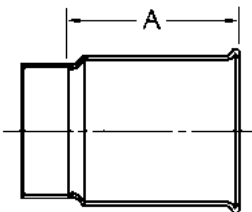
DWV-MJ Soil Pipe Ferrule Copper to Soil Hub
