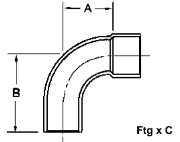
90° Street Elbow-Long Turn Fitting to Copper
