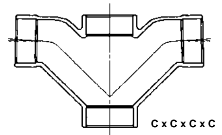
DWV-Double Long Turn TY Copper to Copper to Copper to Copper
