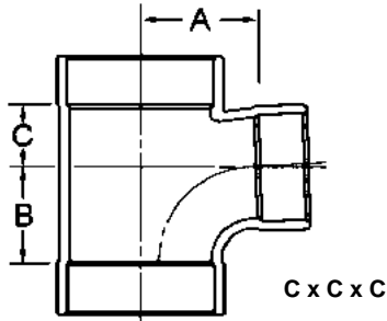
90° DWV TY Copper to Copper to Copper
