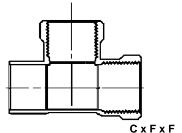
CxFxF Tee Copper to Female NPT to Female NPT
