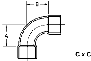
90° Elbow-Long Turn Copper to Copper
