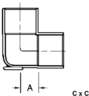
90° CxC Drop Ear Elbow Copper to Copper
